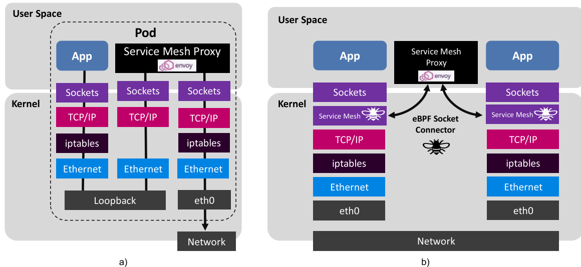
FIGURE 9. How eBPF may reduce the number of service mesh proxies to provide the same services [6], [15], [18], [21].
